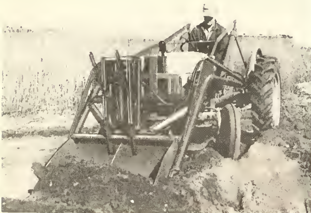
Dirt Bucket (above) and Dozer Blade (below). Two of the quickly interchangeable attachments for the New Idea-Horn hydraulic loader.
